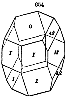
Achmatovsk.
